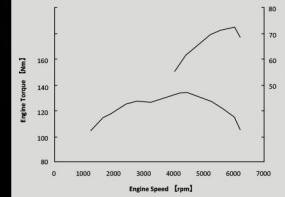
<Engine Performance Curve>
